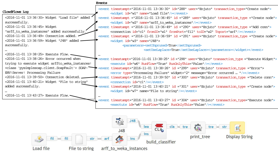
Figure 1: Top: Example of a log using ClowdfloWS and its formatting into events. Complete information about events is extracted by means of http/network inspector tools. Bottom: the corresponding data-to-knowledge flow finally completed by the data scientist.
