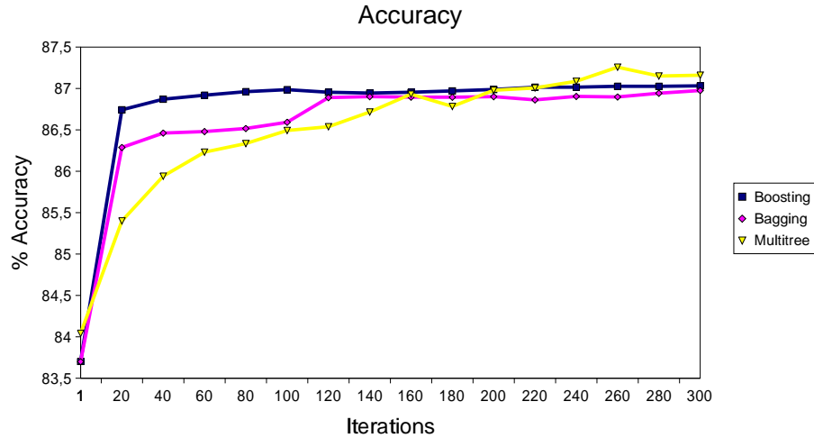
Fig. 2. Accuracy comparison between ensemble methods.
