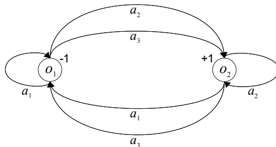
Figure 6: A simple automaton.
